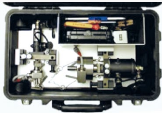
Online testing accessories with 1kN and 20kN bridge
